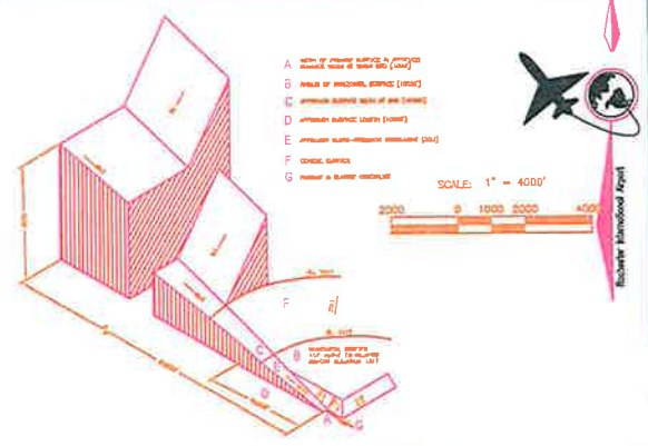
PART 77 IMAGINARY SURFACES ISOMETRIC VIEW
